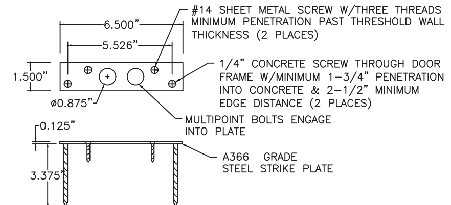
2 BOTTOM STRIKE PLATE
