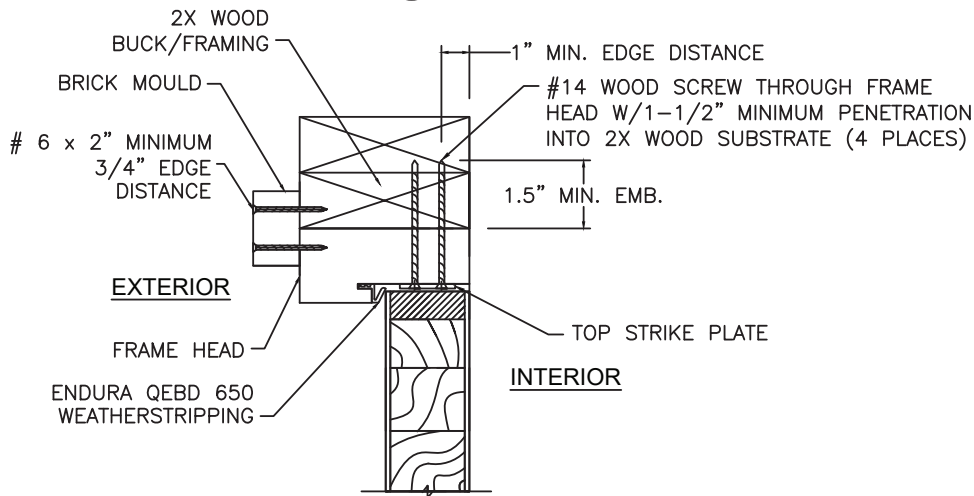
1 TOP STRIKE PLATE
