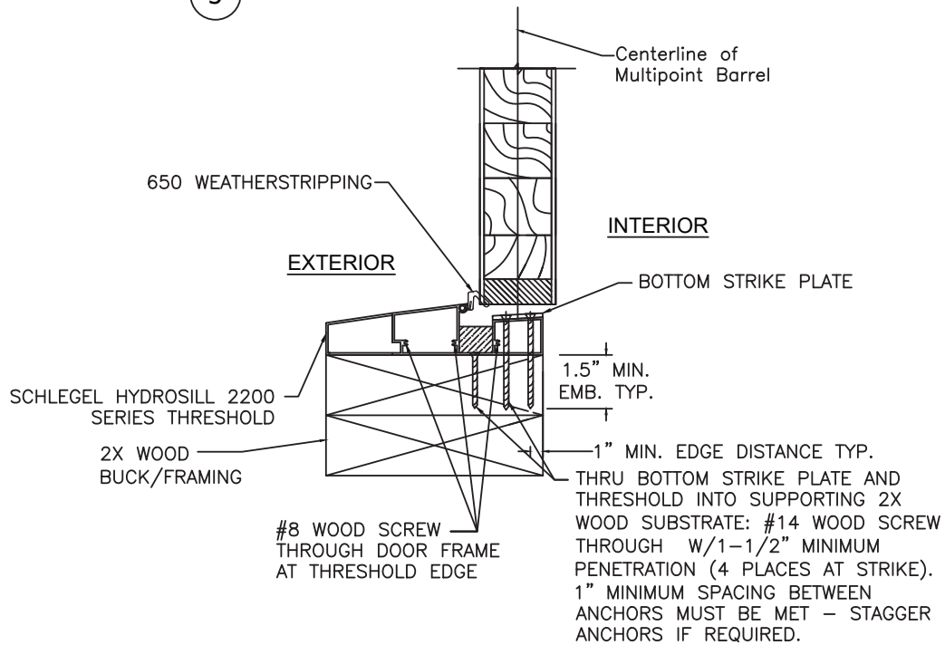
4 THRESHOLD SECTION AT STRIKE PLATE
